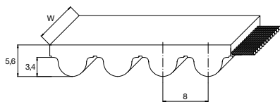
TOOTH PROFILE ACCORDING ISO 13050
